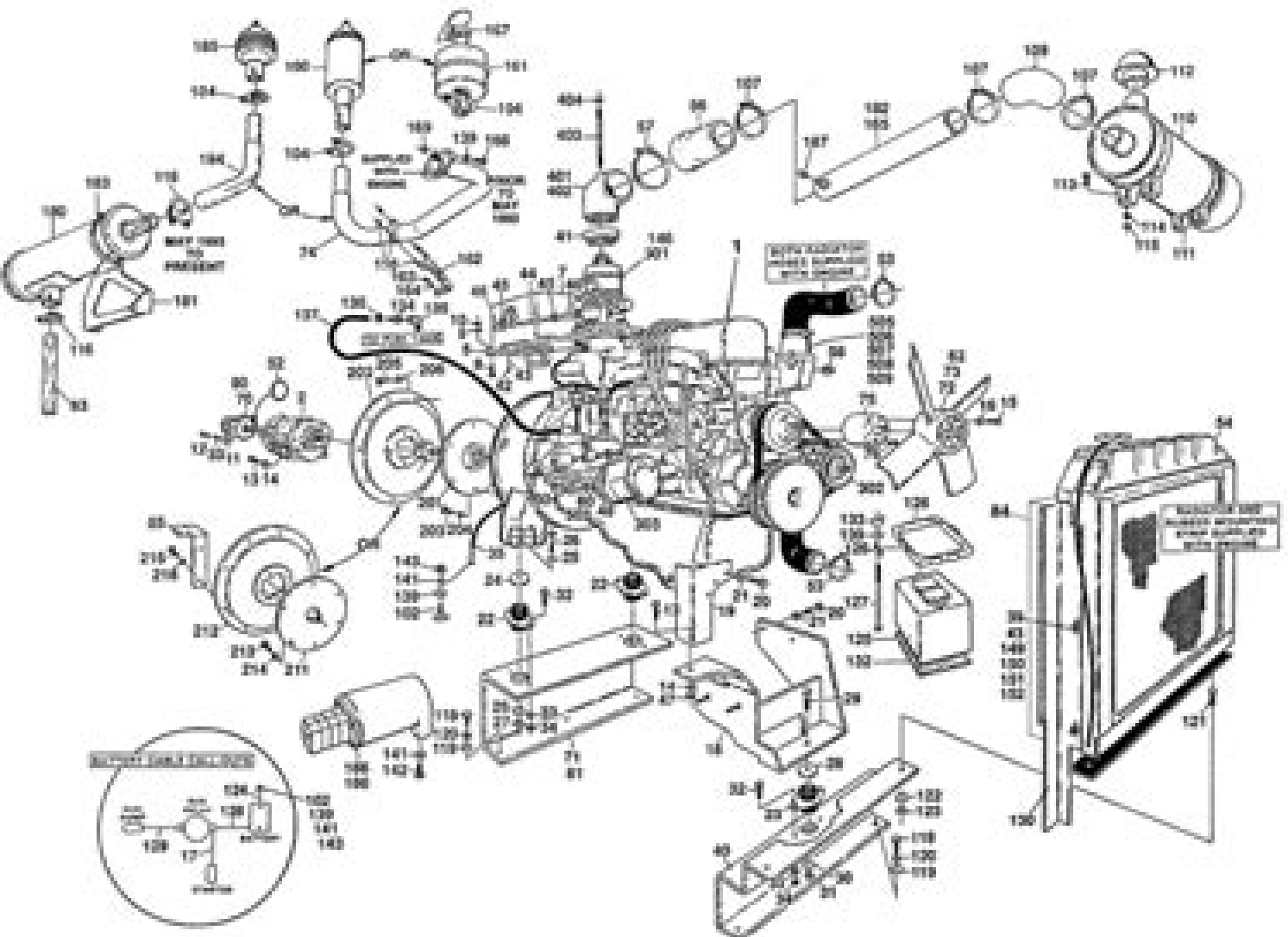
FIGURE 2-17. FORD ENGINE INSTALLATION
