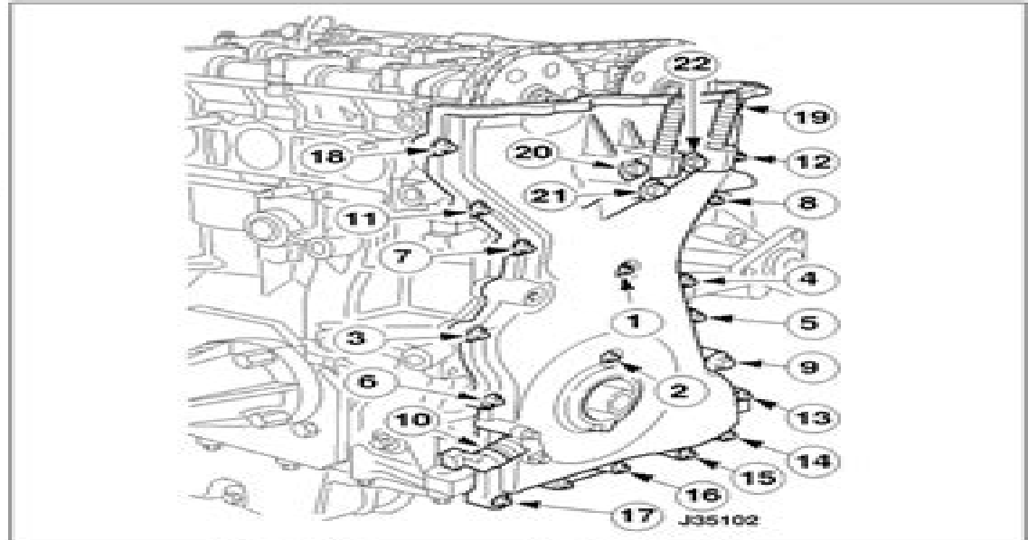
9.13b Tightening sequence for the timing chain cover
