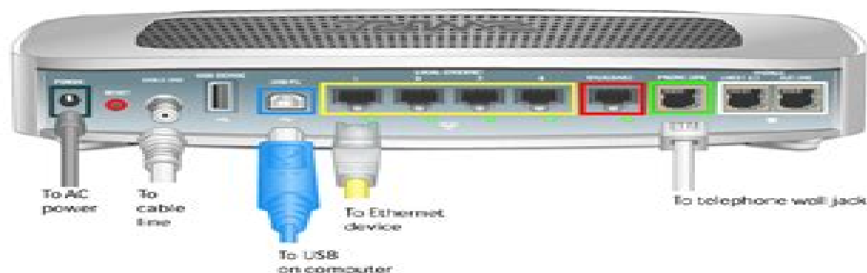
Figure 1. 3800HGV-B, Rear View
