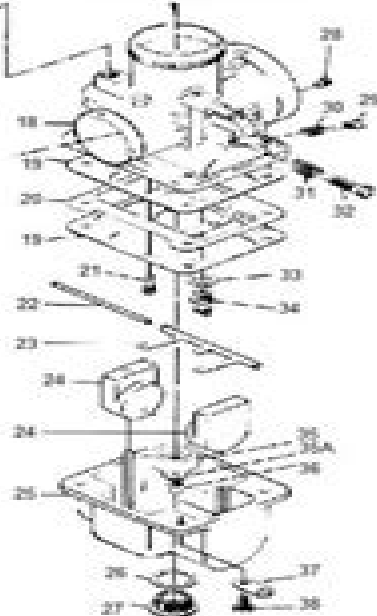
Diagram A Exploded view of a SPIGOT MOUNT TYPE MIKUNI CARBURETOR
