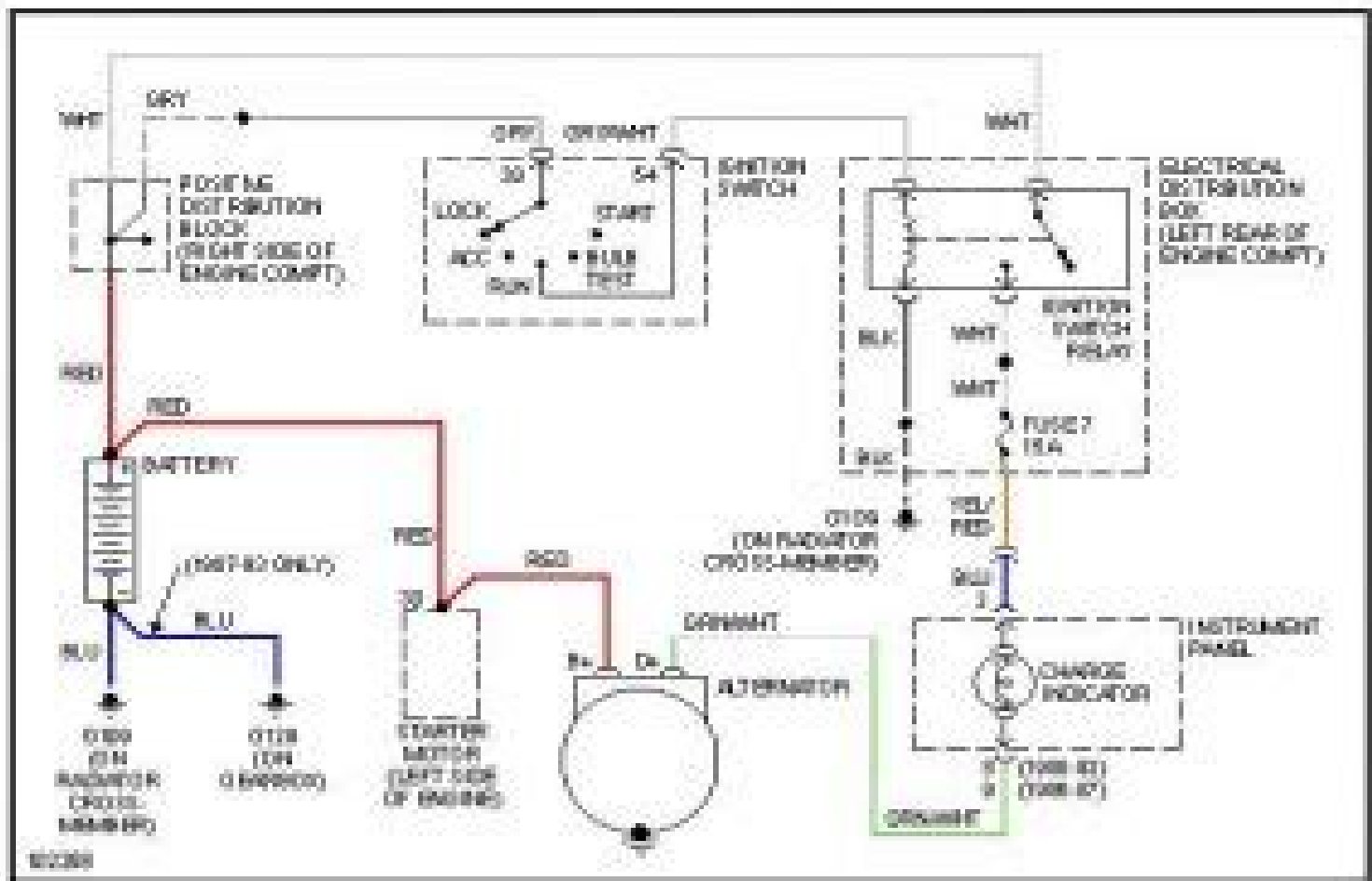
1990 Saab 900-Fig. 14: Charging Circuit
