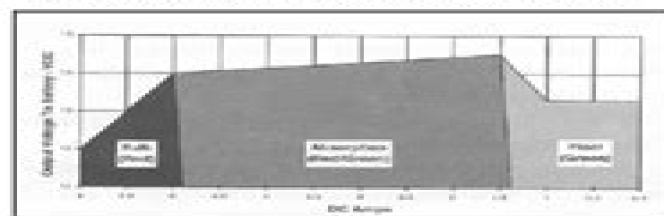
Figure 2-6 Charging Method
