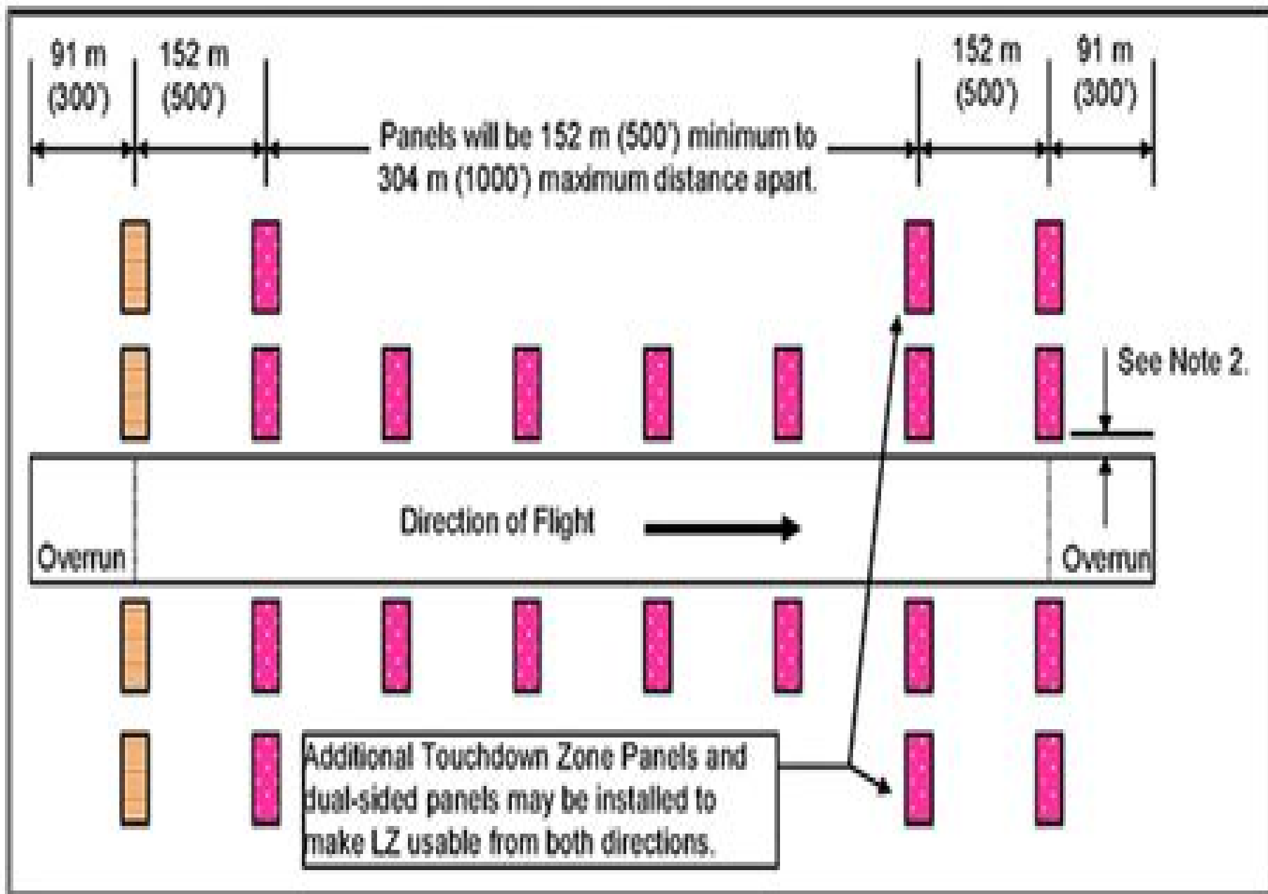
Figure 7-8a – Airfield Marking Pattern 1 (Day)
