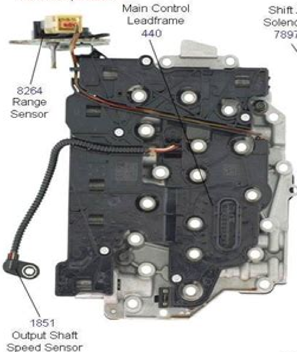
Front view with Main Control Leadframe
