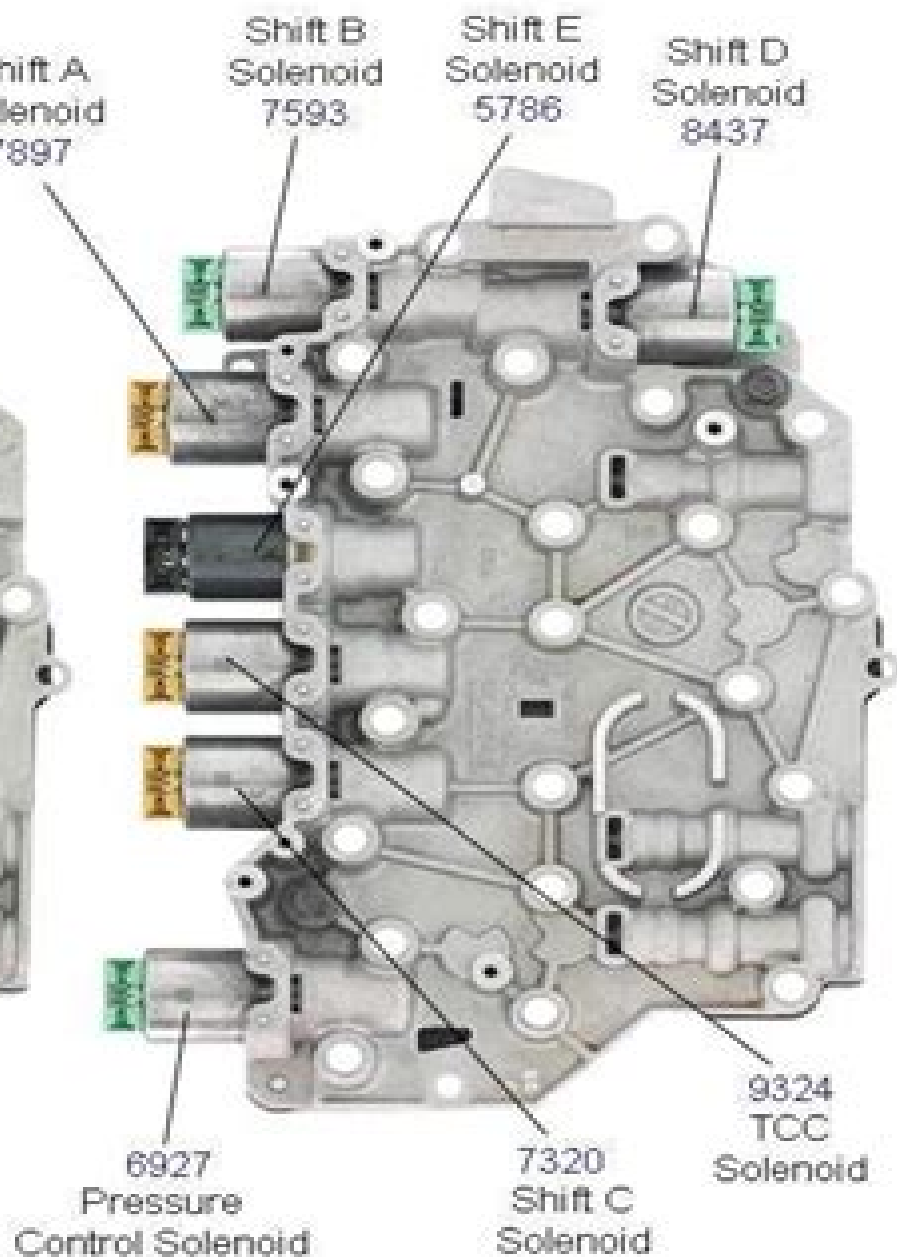
Front View Without Main Control Leadframe
