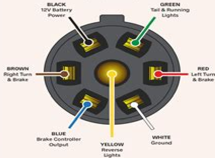
Plug Side
