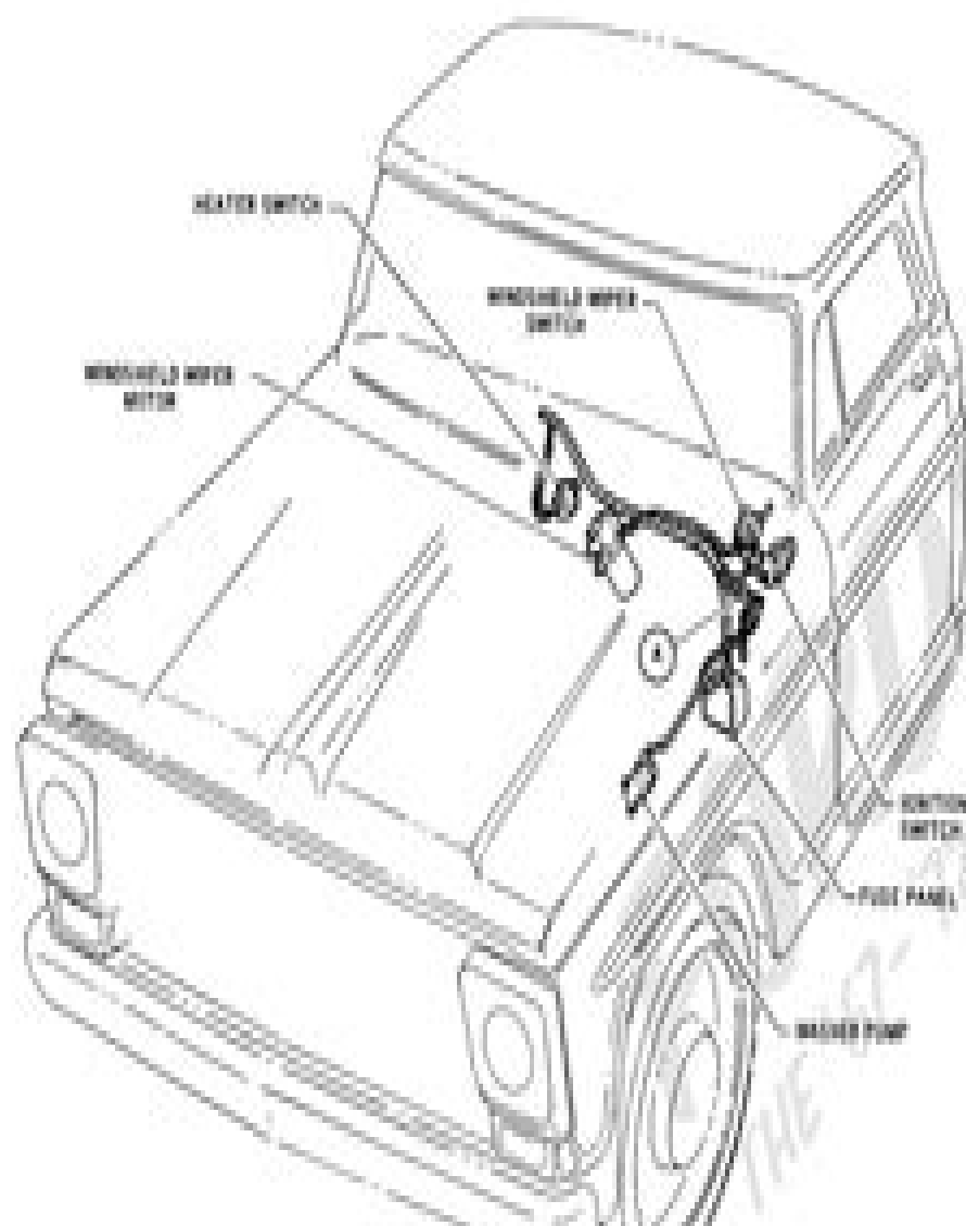
1967 F-100 THRU 350 SERIES TRUCK WINDSHIELD WIPER AND WASHER
