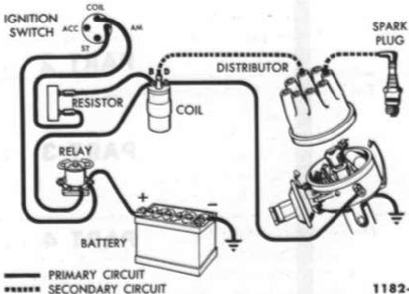
Fig. 1—Ignition Circuit—Typical
