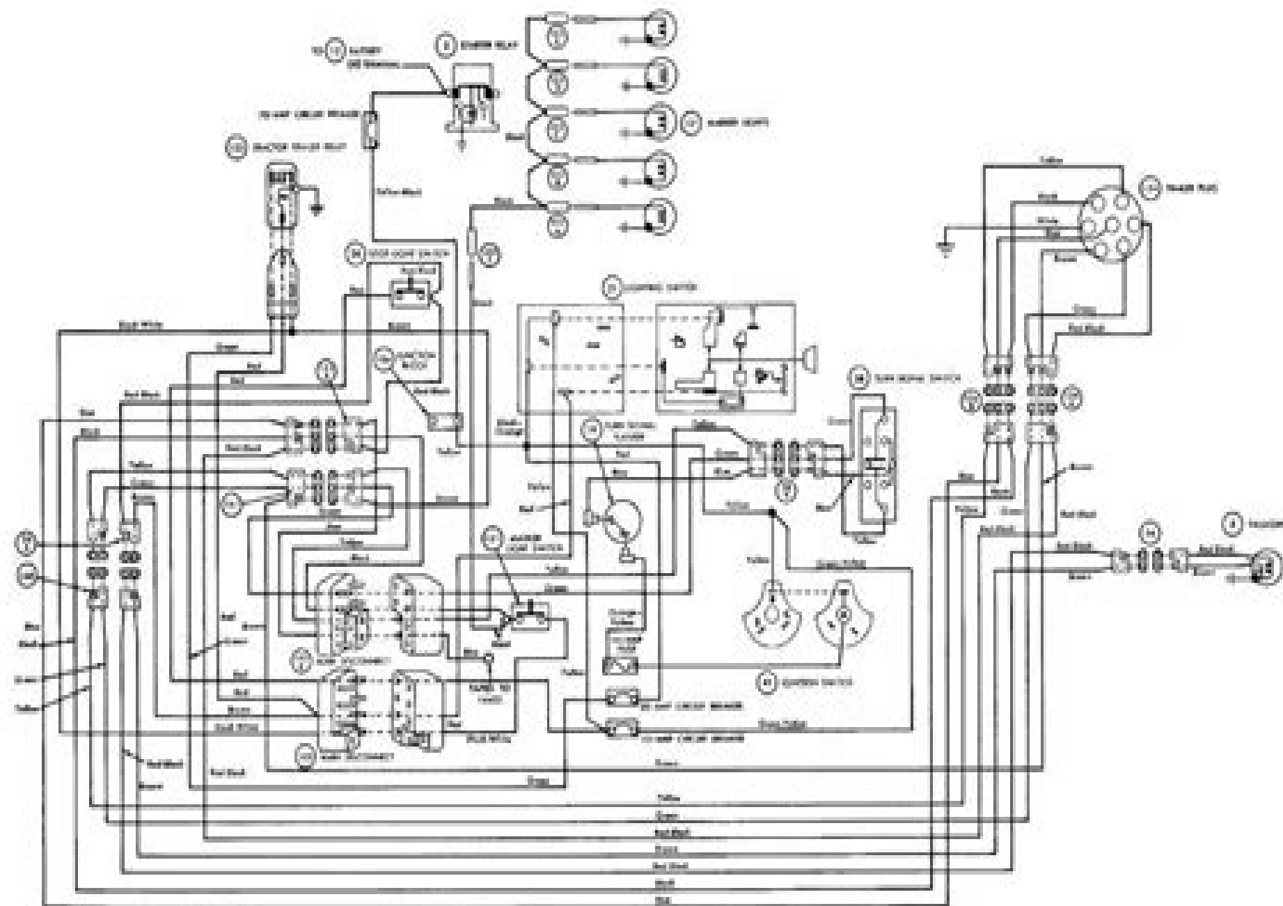
1964 B-, F- AND T-SERIES TRUCKS TRACTOR TRAILER MARKER LIGHTS SCHEMATIC
