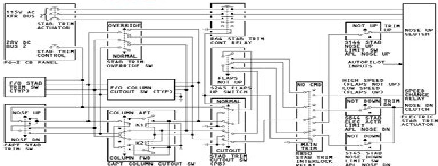
HORIZONTAL STABILIZER TRIM CONTROL SYSTEM - ELECTRIC TRIM - FUNCTIONAL DESCRIPTION
