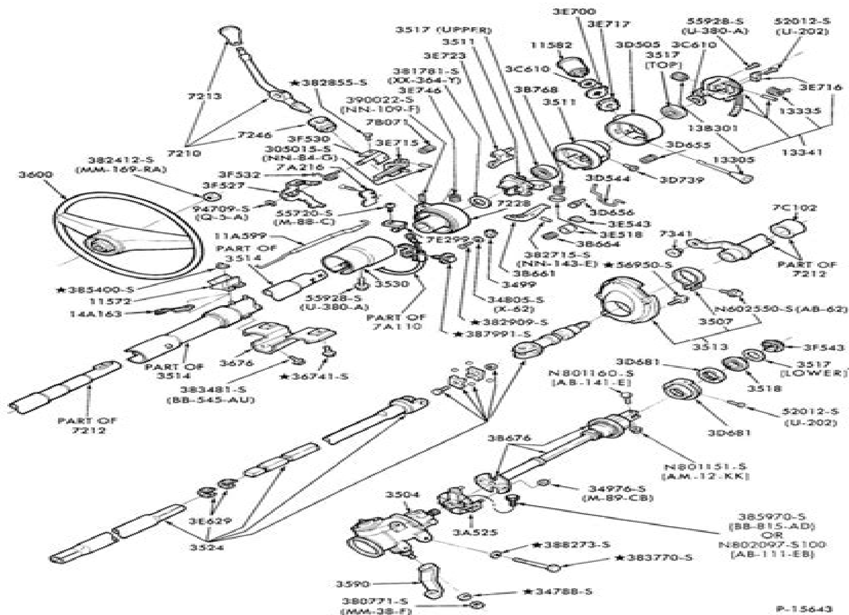
STEERING COLUMN and SHIFT CONTROL SELECTOR MECHANISM — TILT WHEEL
