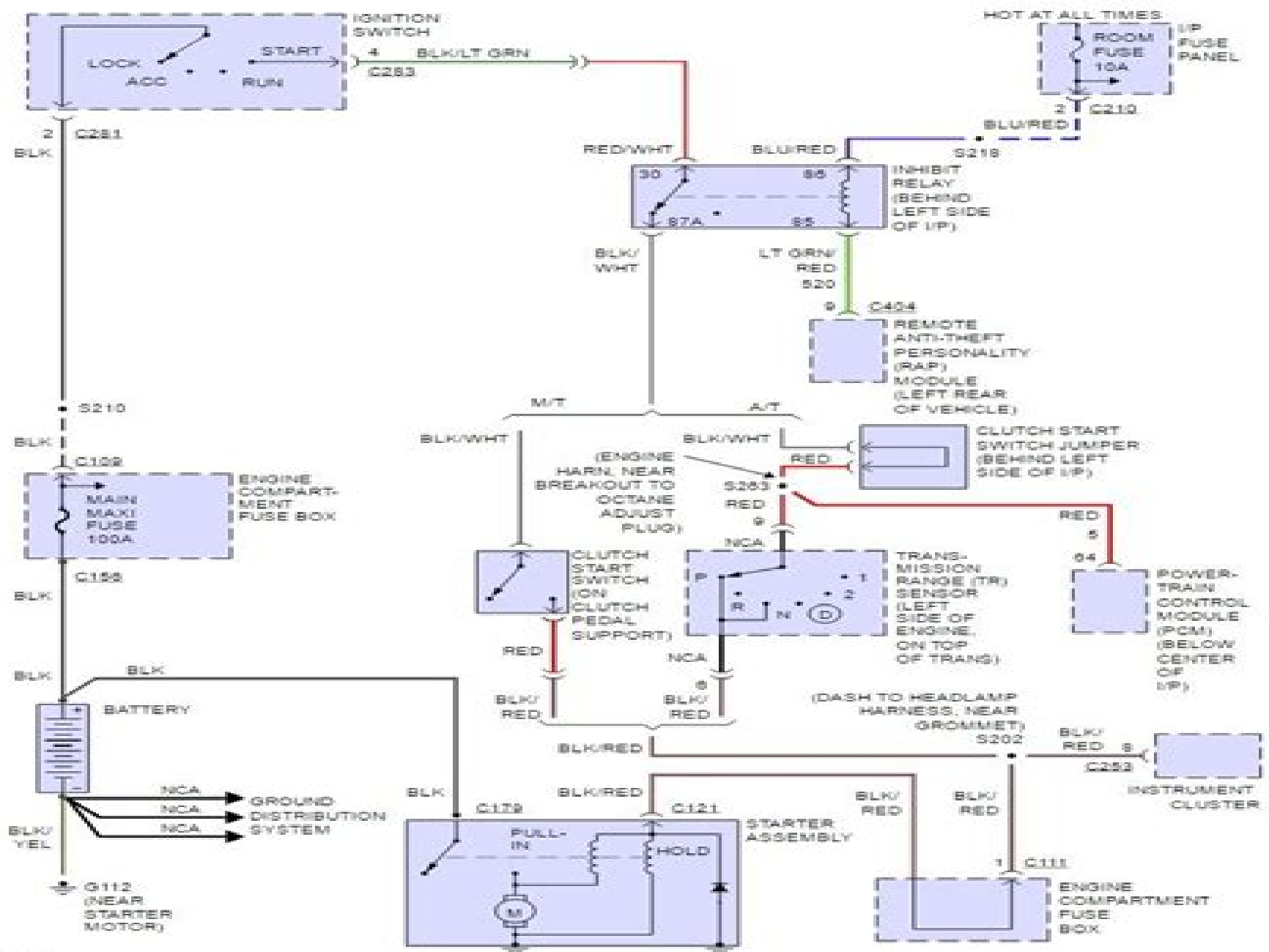
Fig 2: Starting Circuit
