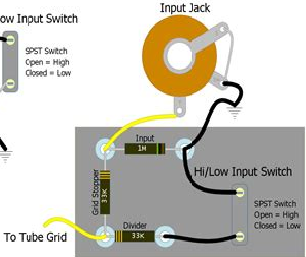
Circuit Board
