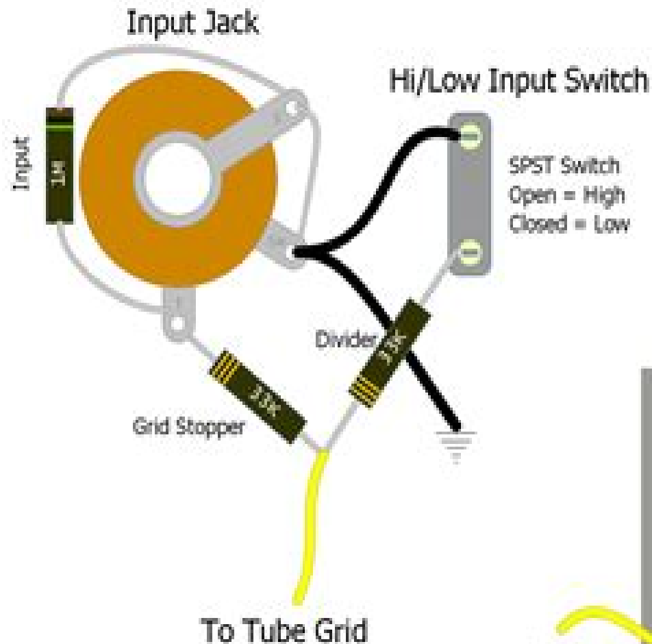
Jack Mounted
