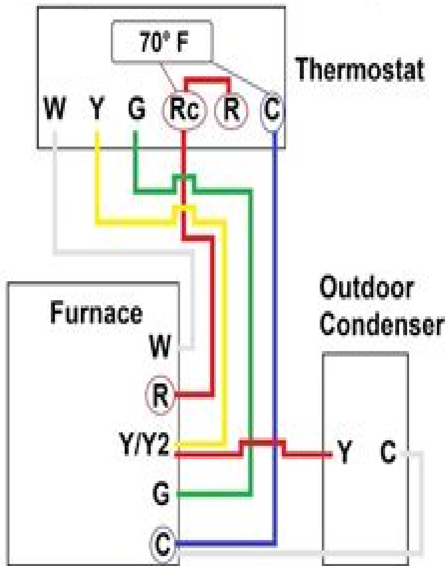
Wiring Diagram for a Furnace and A/C System
