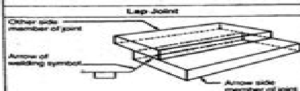
Basic Joints—Identification of Arrow Side and Other Side of Joint
