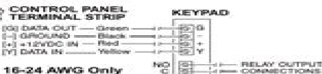
Detail A
