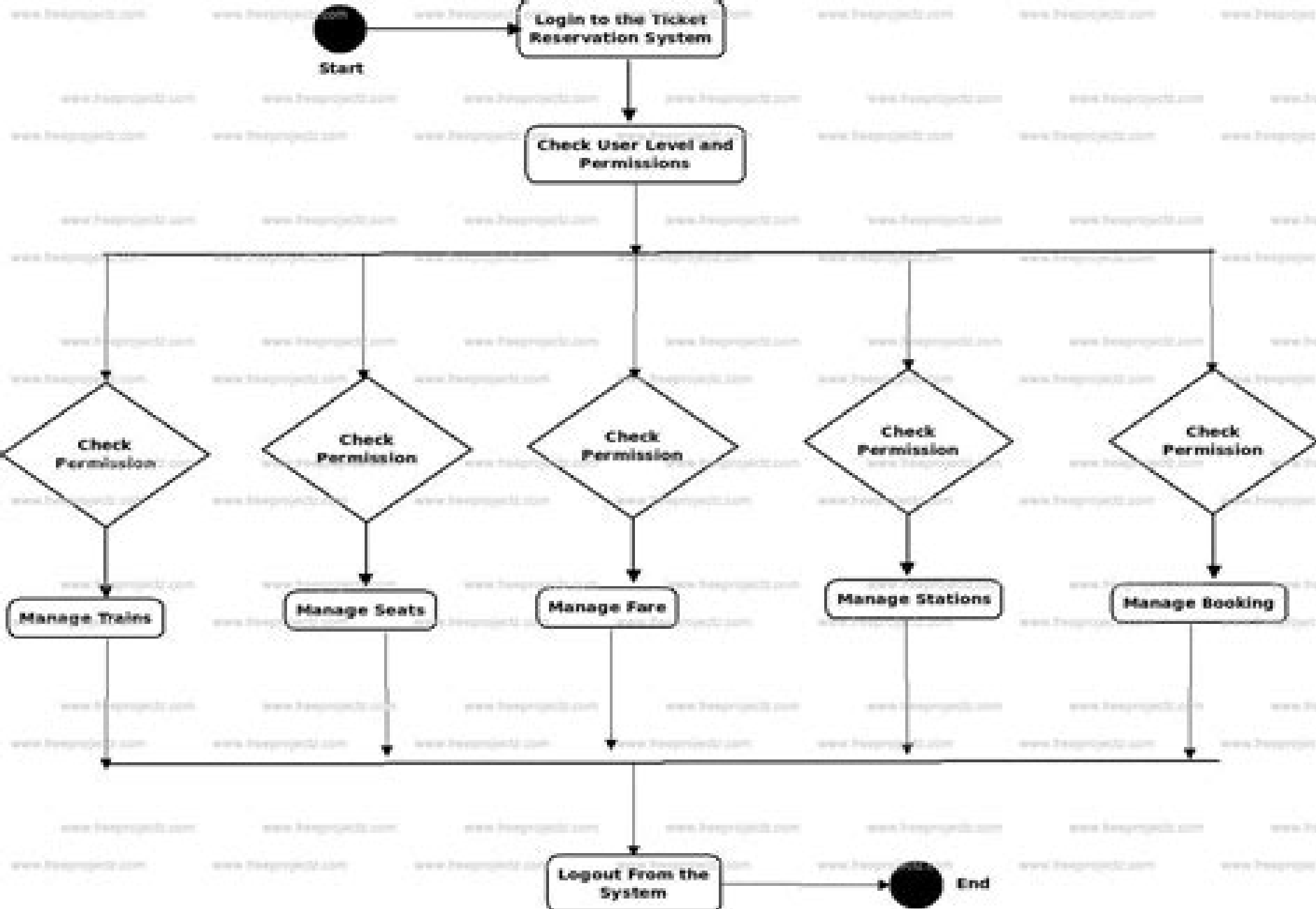
Activity Diagram for Ticket Reservation System
