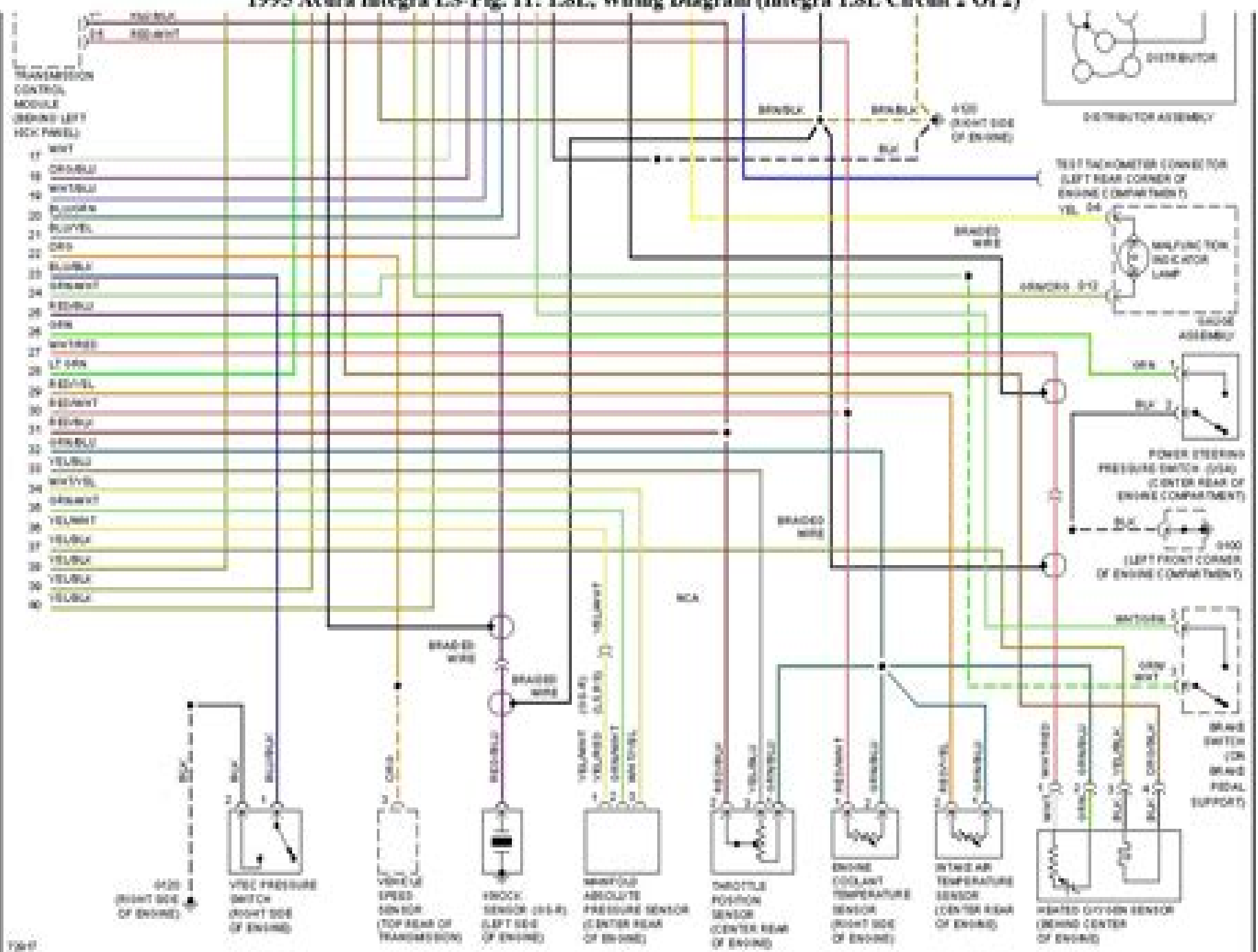
1995 Acura Integra LS- Fig. 11: L&L Wiring Diagram (Integra L&L Circuit 2 Of 2)
