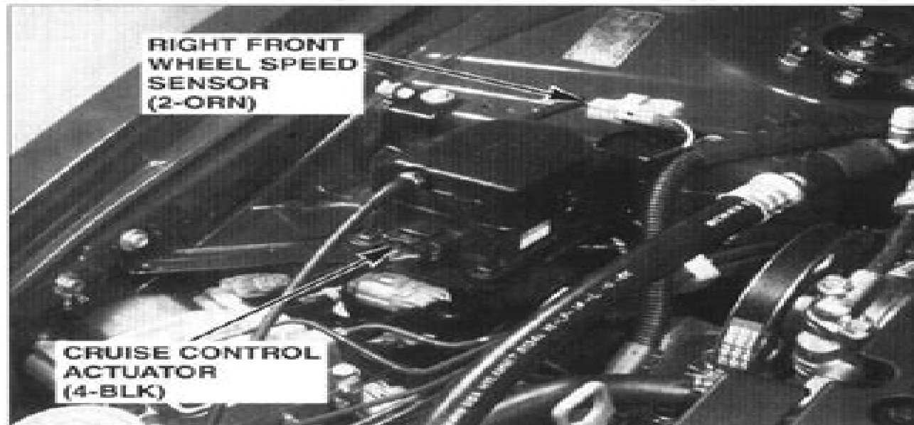
8. Right Side of Engine Compartment (Type S – A/T)
