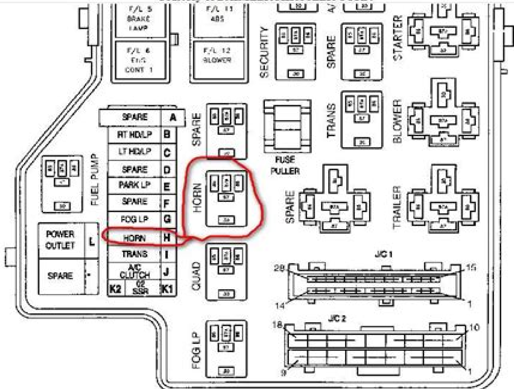
Fig. 2: Identifying Power Distribution Center Fuses, Circuit Breakers &amp; Terminals
