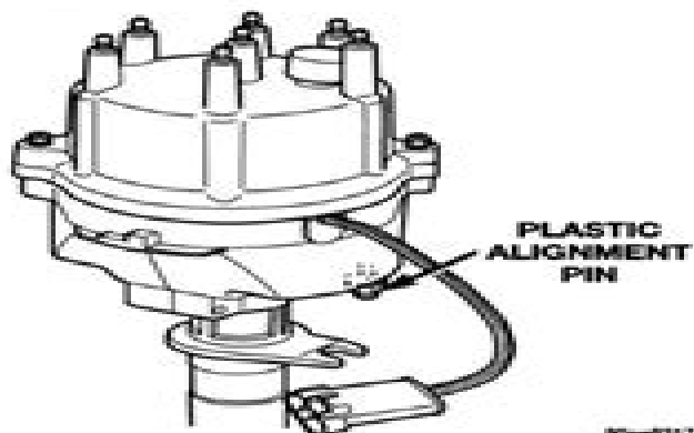
Fig. 30 Plastic Alignment Pin
