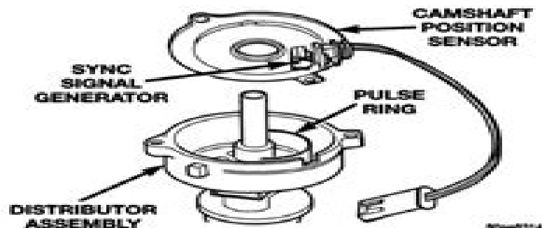
Fig. 29 Camshaft Position Sensor—Typical (3.9/5.2/5.9L Shown)
