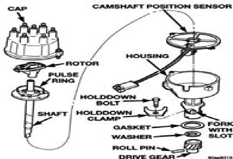
Fig. 31 Distributor—2.5L Engine—Typical
