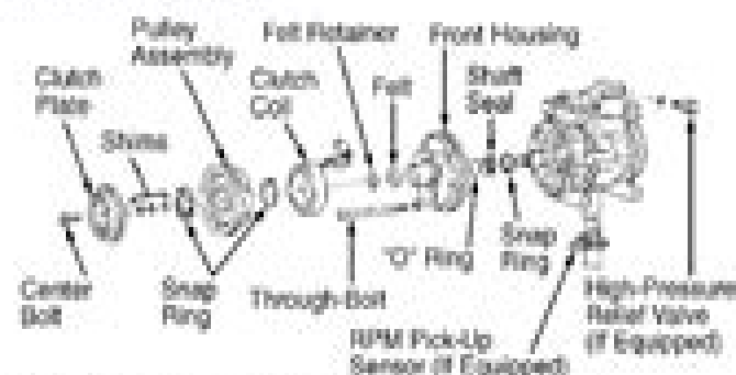
Fig. 3: Compressor (Nippondenso 10PA17C, 10PA15 & 10PA20 Are Similar) Courtesy of Mitsubishi Motor Sales of America
