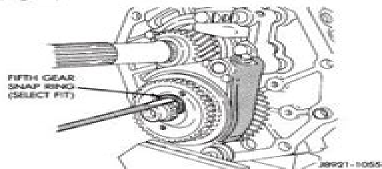
Fig. 21 Removing Fifth Gear Snap Ring
