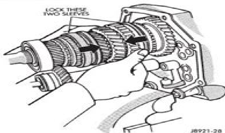
Fig. 20 Locking Mainshaft Gears
