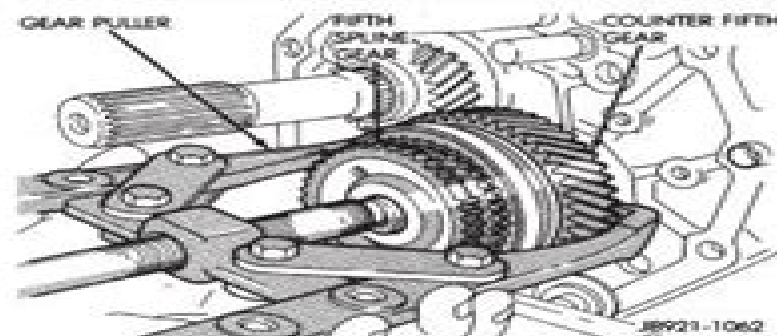
Fig. 22 Removing Fifth Gear Assembly
