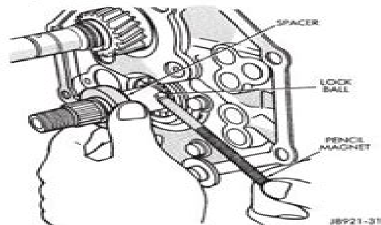
Fig. 23 Spacer And Lock Ball Removal
