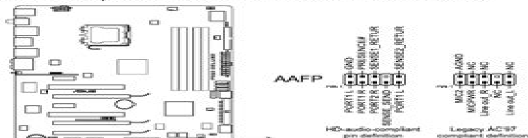
P5Q3 DELUXE Analog front panel connector
