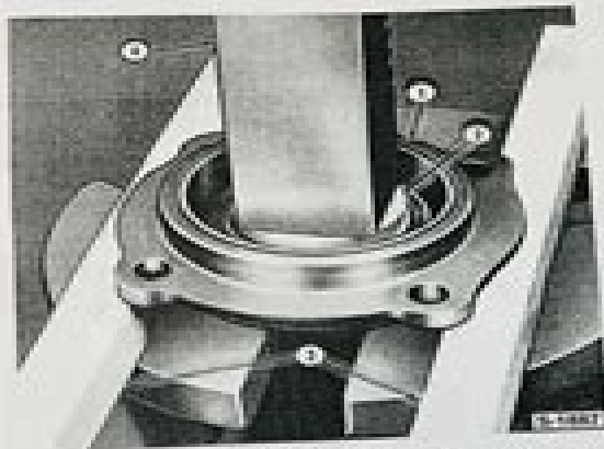
Figure 305 Output Shaft Bearing Retainer — Seal Removal 1. Bearing Retainer 3. Support Blocks 2. Deep Flange — Tool No. 9210 4. Press
