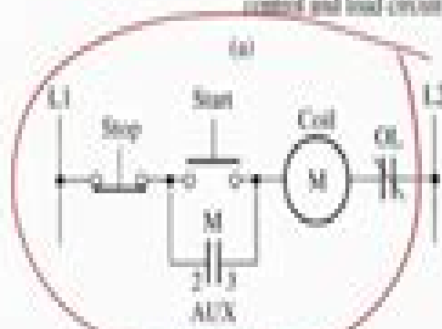
Ladder diagram of control circuit
