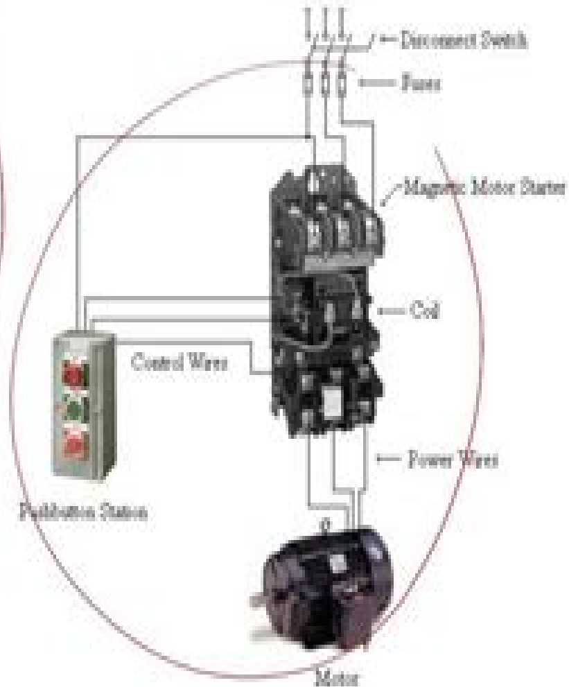
Three-phase Motor wiring diagram of control and load circuit
