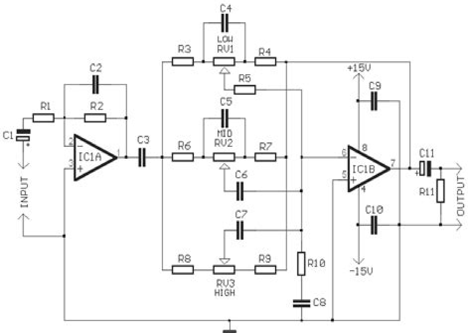
3 Band Graphic EQ.
