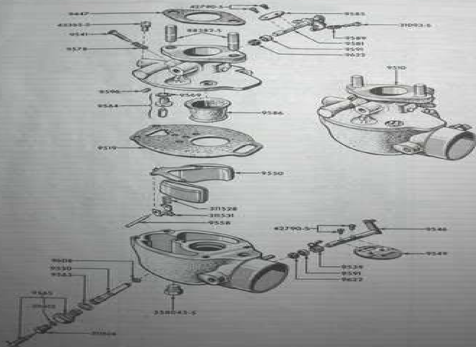
FIG. 982 - CARBURETOR ASSY. - 1958/
