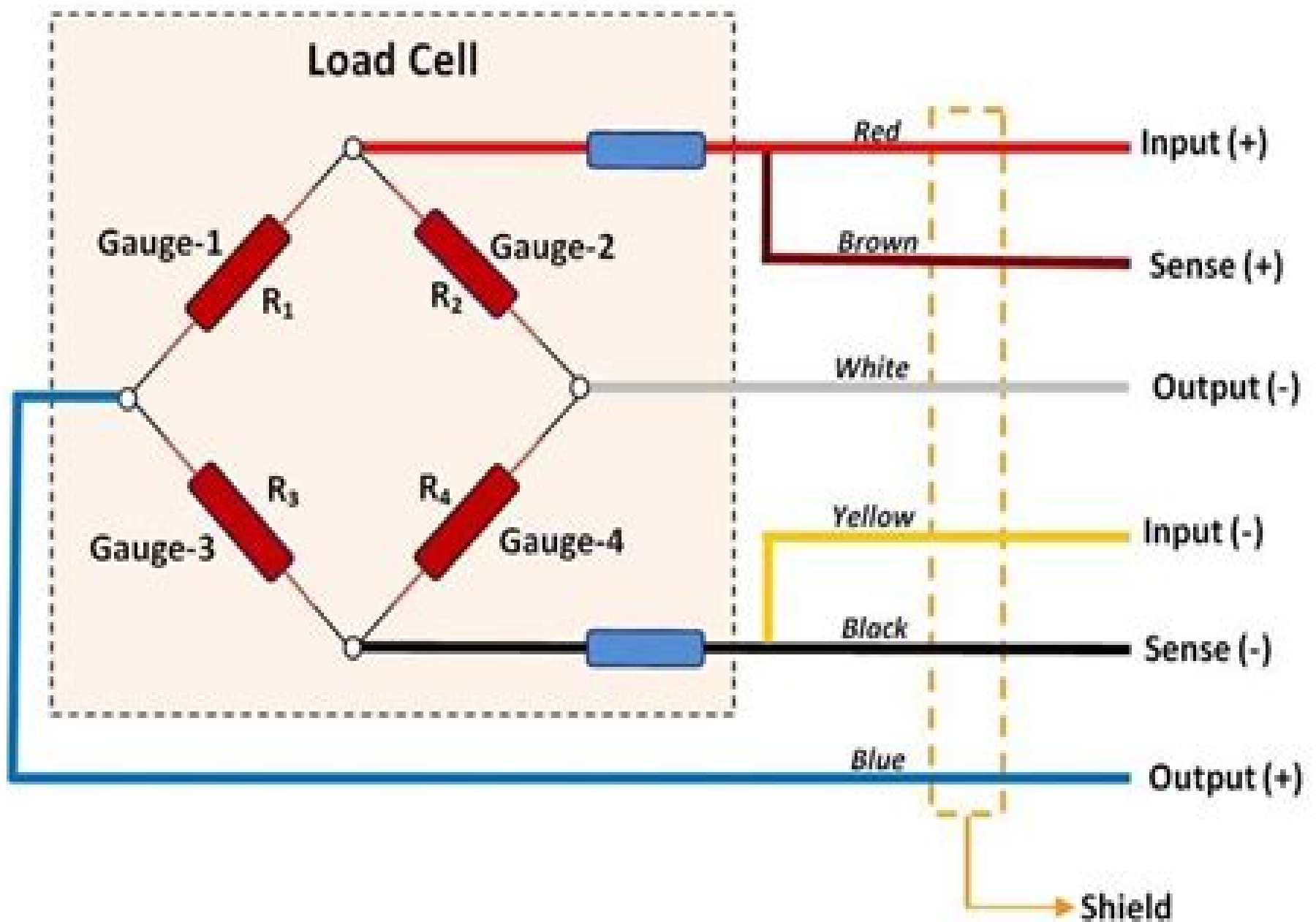
6 wire Load cell wiring diagram
