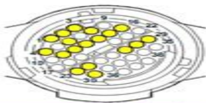
38 pin Iveco proprietary diagnostic connector for Autocom scanner
