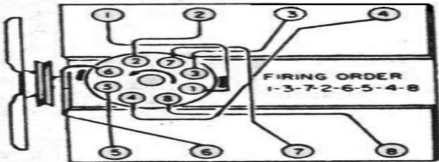
standard rotation (LH) Ford 351w V8
