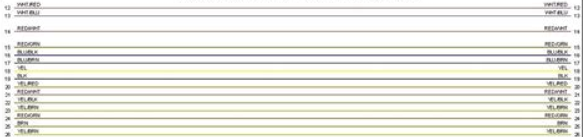
2005 BMW X5-Fig. 116: Premium Radio Circuit, W/ Top HiFi Radio (2 of 3)
