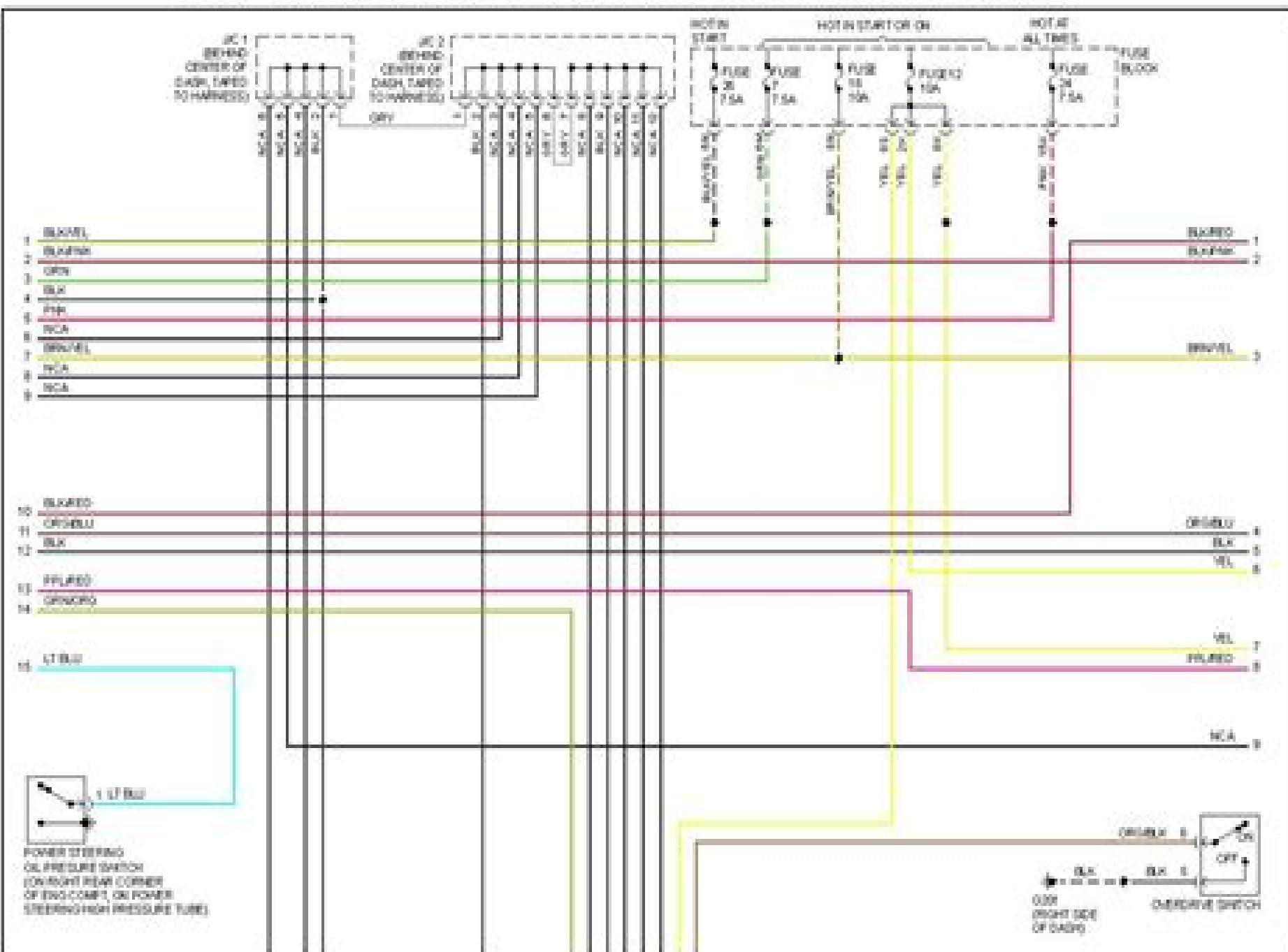
1998 Nissan Sentra-Fig. 12: 1.6L, Engine Performance Circuits (2 of 3)
