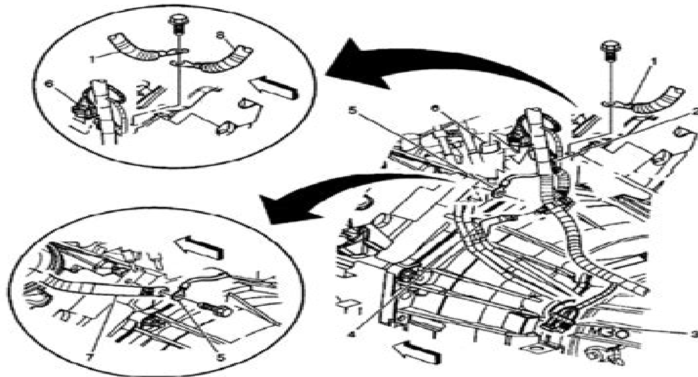
Fig. 5: Rear Of Engine (4.8L, 5.3L & 6.0L) Courtesy of GENERAL MOTORS CORP. 2006 Cadillac Escalade
