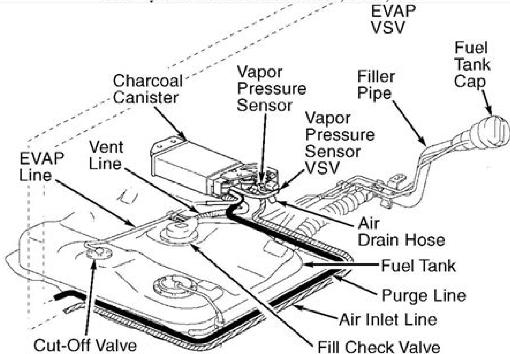
Fig. 14: Vacuum Diagram (Corolla - 2 Of 3)
