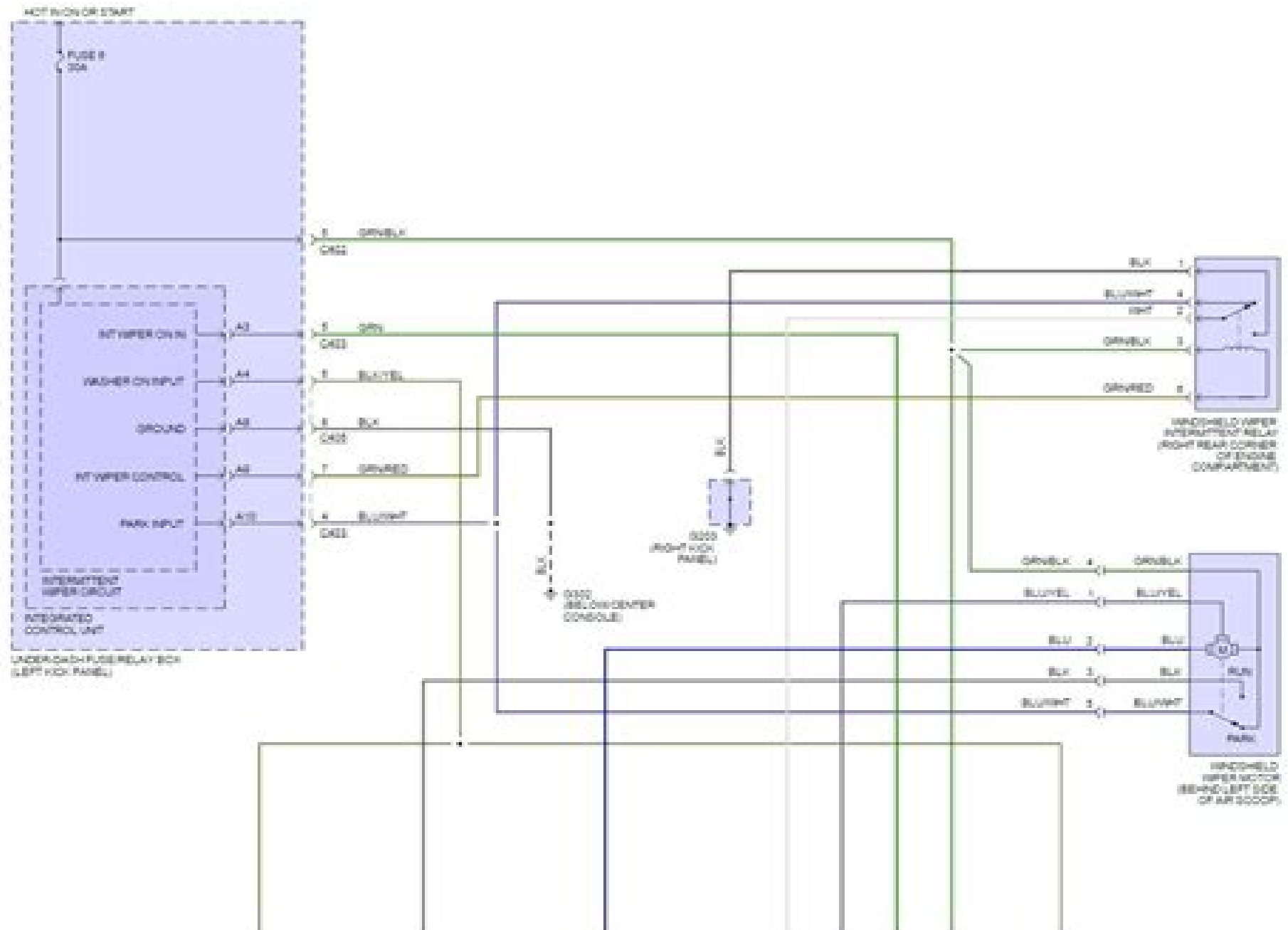
Fig 1: Front Wiper/Washer Circuit
