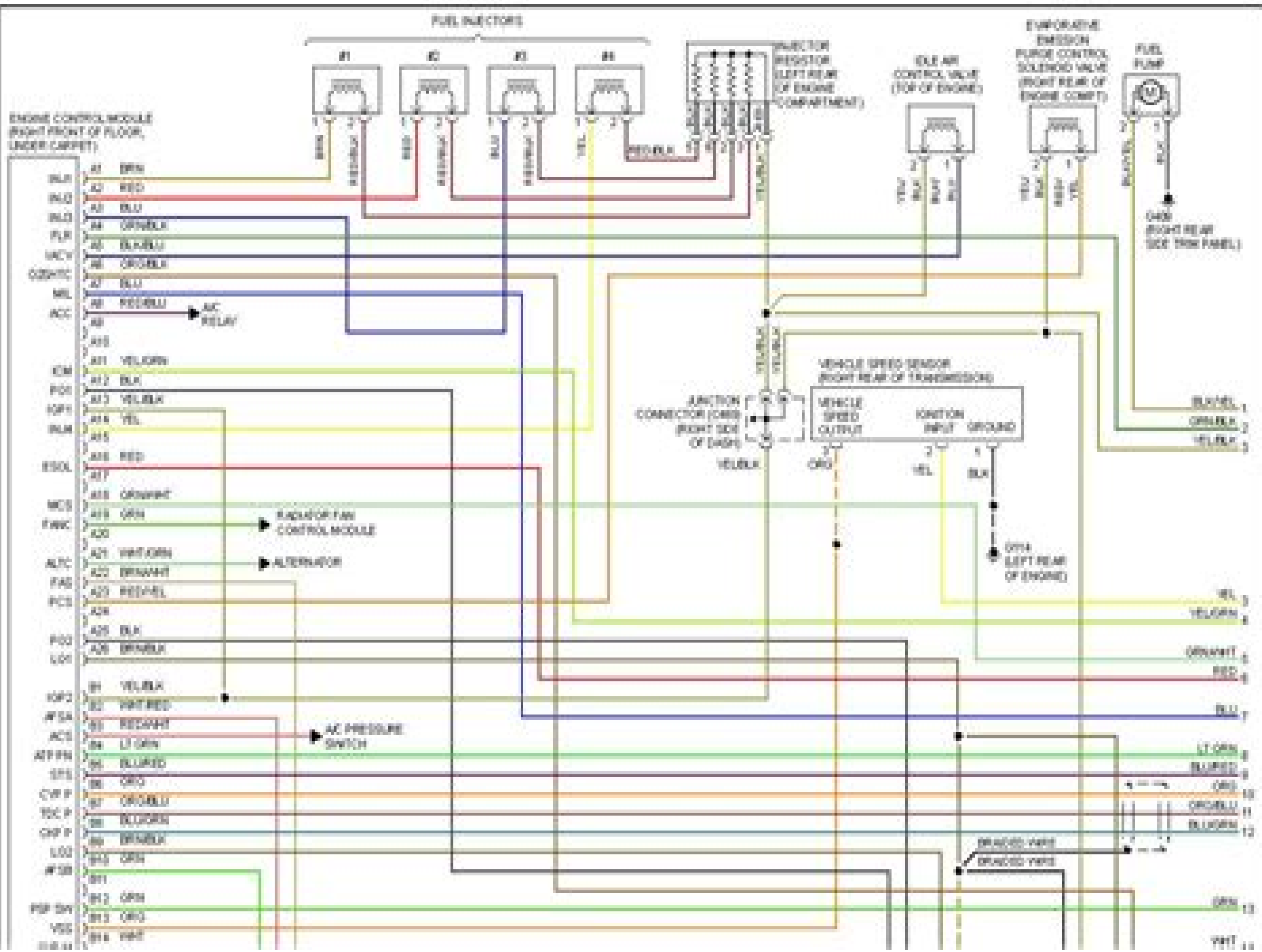
1995 Honda Odyssey EX-fig. 9-2.9, Engine Performance Circuits (1 of 2)
