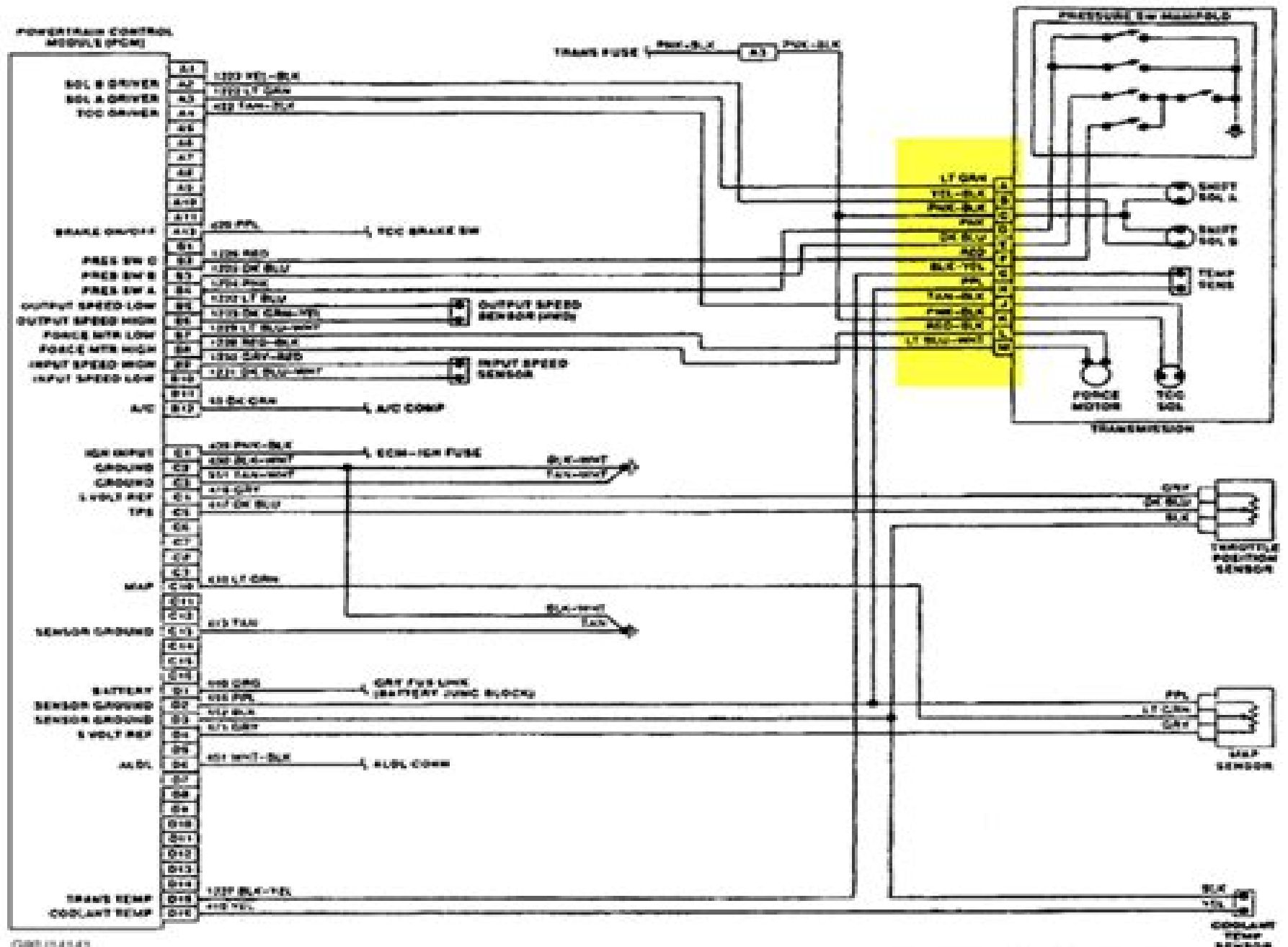
Fig. 70: Wiring Diagram ("C" & "K" Series - Gasoline Engine)
