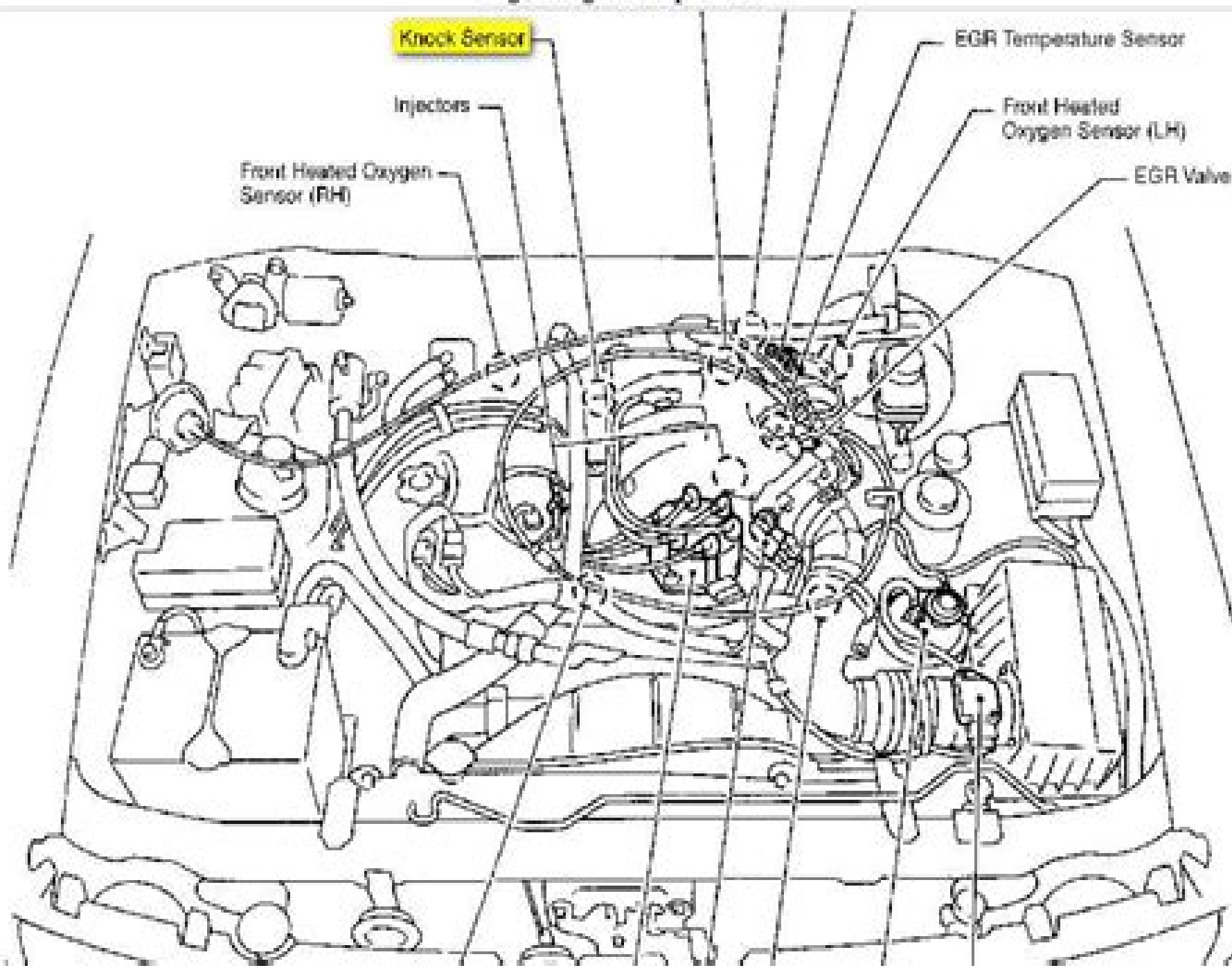
Fig. 2: Engine Compartment
