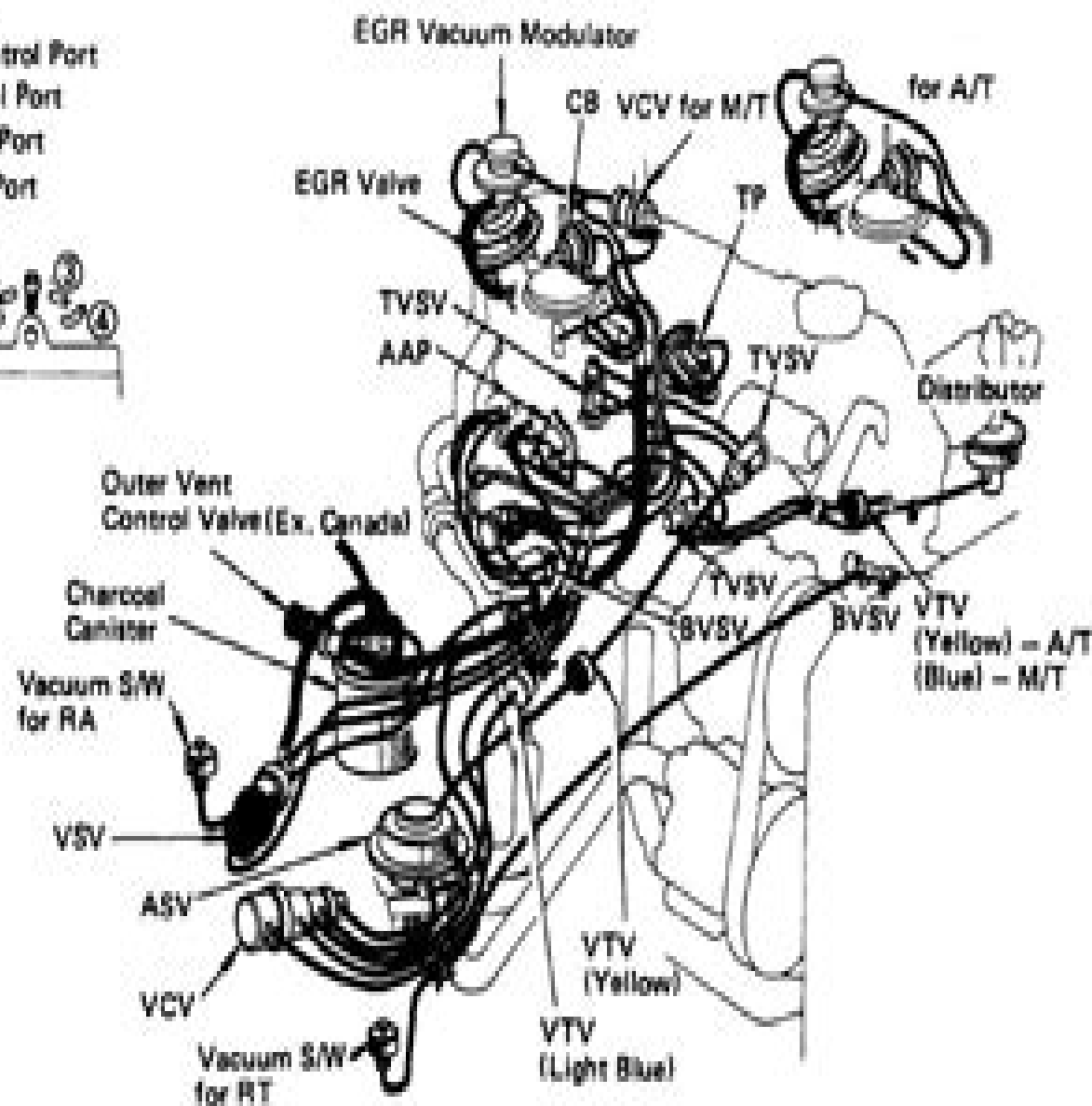
Fig. 61: 1978 Celica & Corolla (20R Engine) Exhaust Emission System (California)
