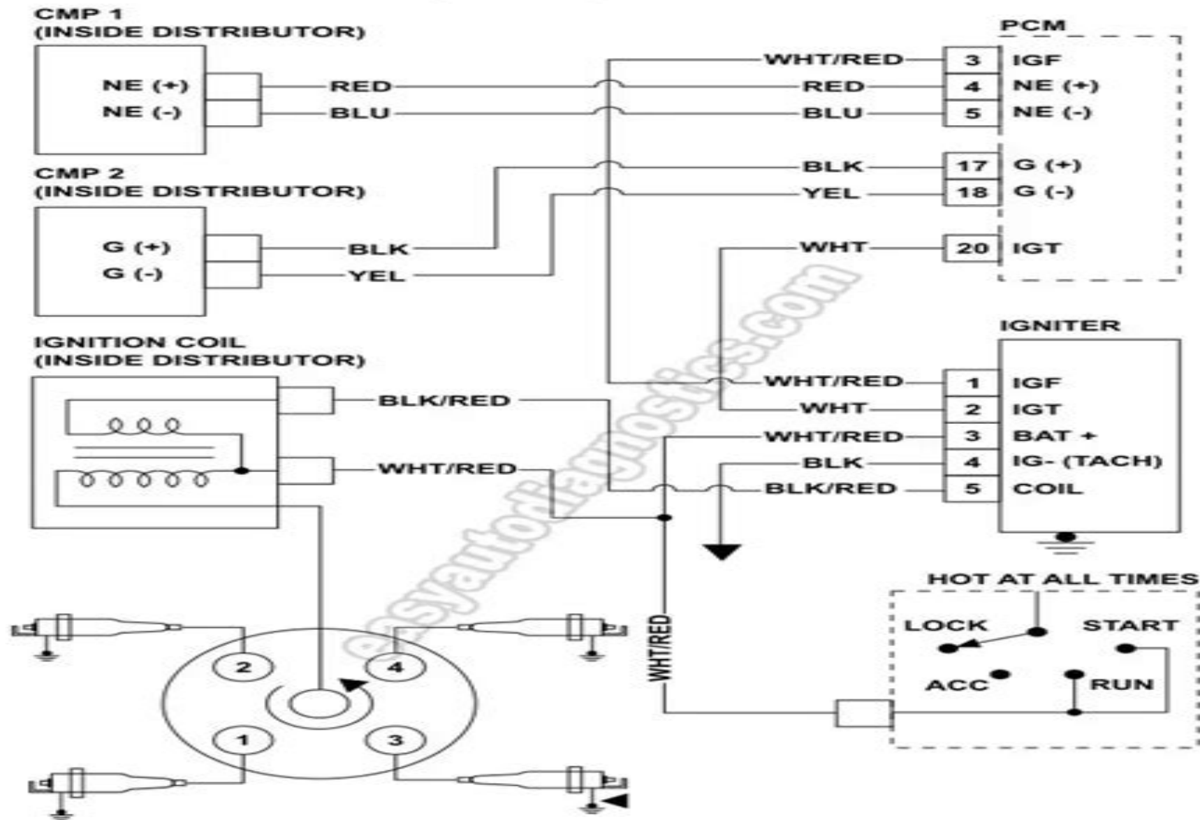
IGNITION SYSTEM WIRING DIAGRAM (1992-1995 2.2L TOYOTA CAMRY)
