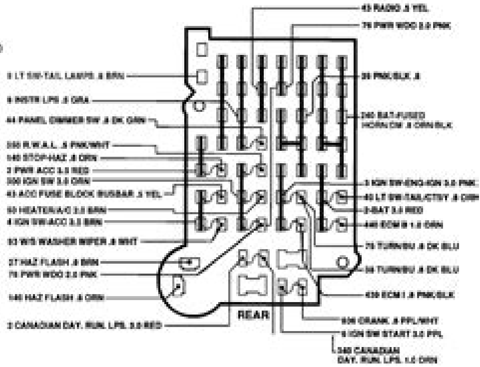
FUSE INFORMATION
