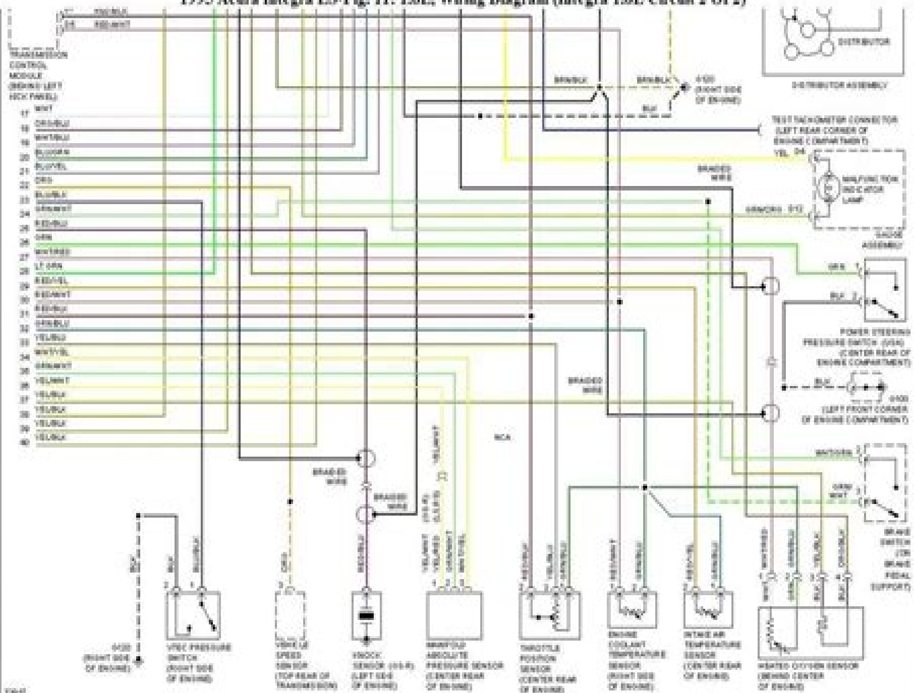
1995 Acura Integra LS Fig. 11: 1.8L, Wiring Diagram (Integra 1.8L Circuit 2 Of 2)
