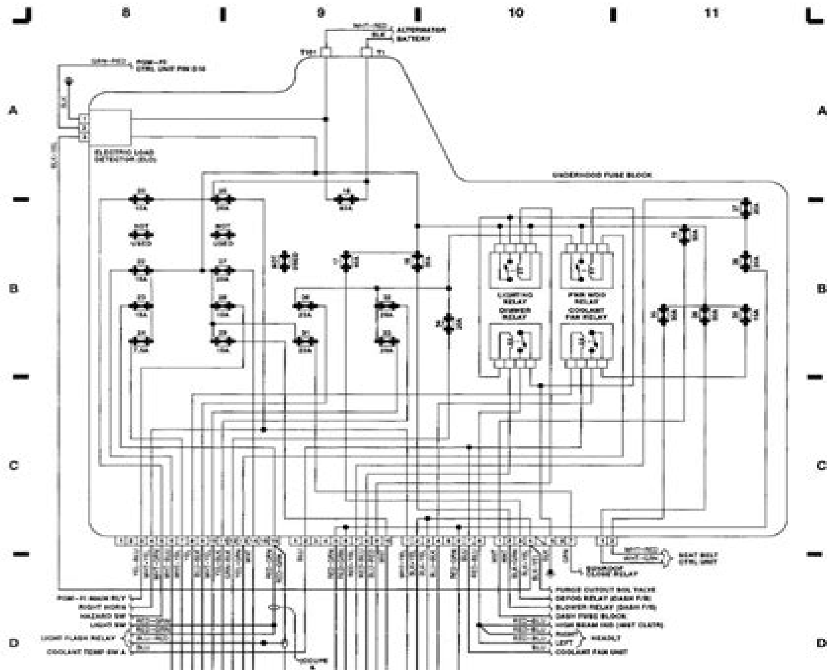
Fig 3: Underhood Fuse Block (Grds 8-11)
