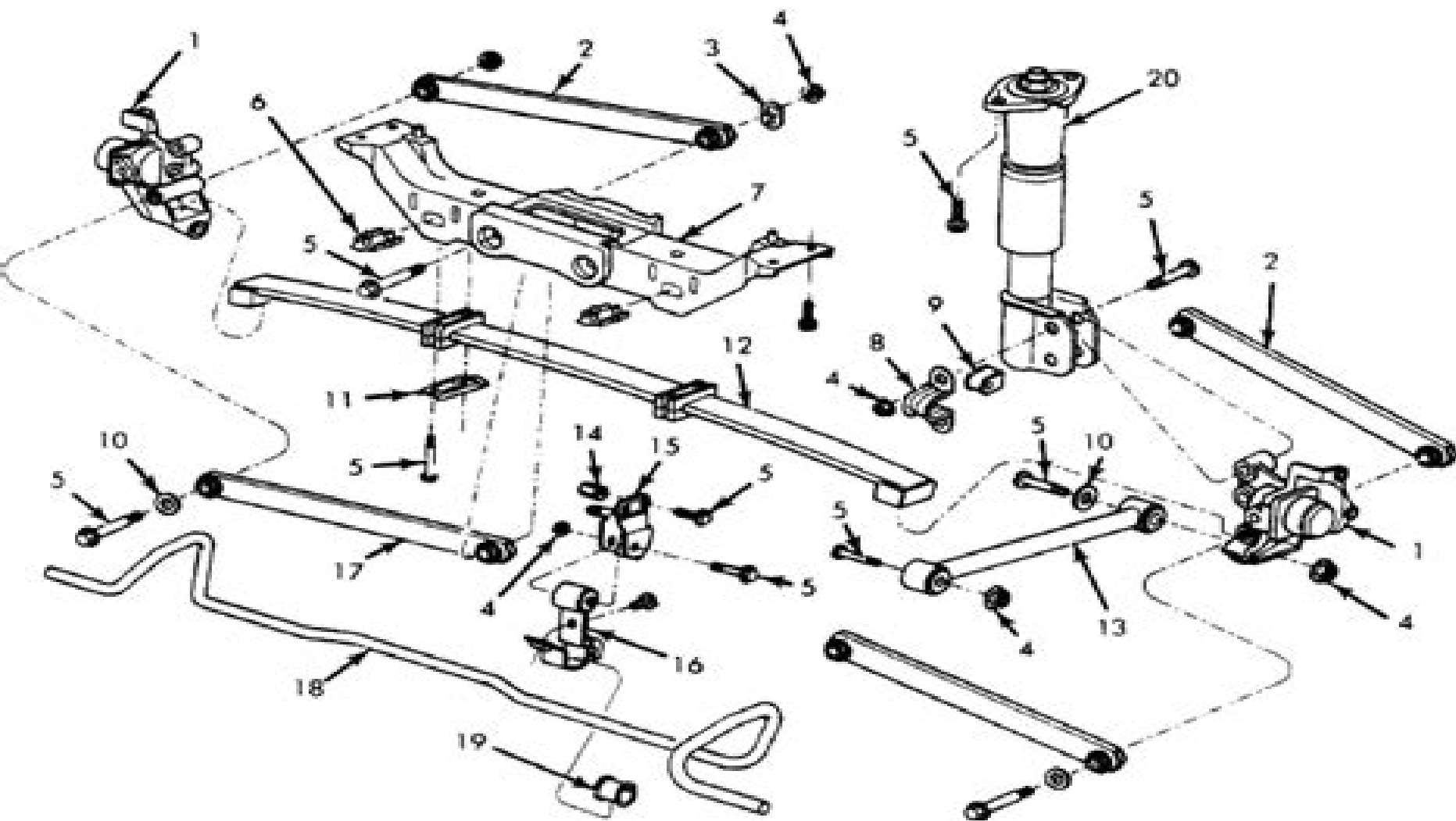
Fig. 5: Exploded View of "W" Body Rear Suspension Courtesy of GENERAL MOTORS CORP.
