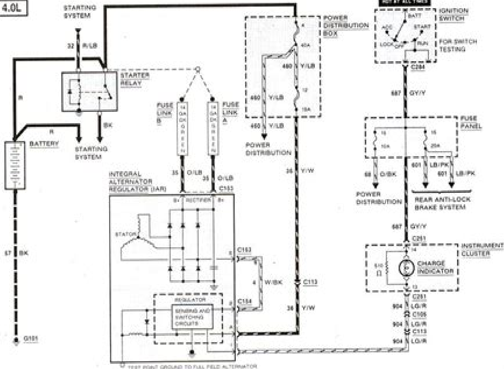
Charging system – late models (typical – 1991 shown) (part 1 of 2)
