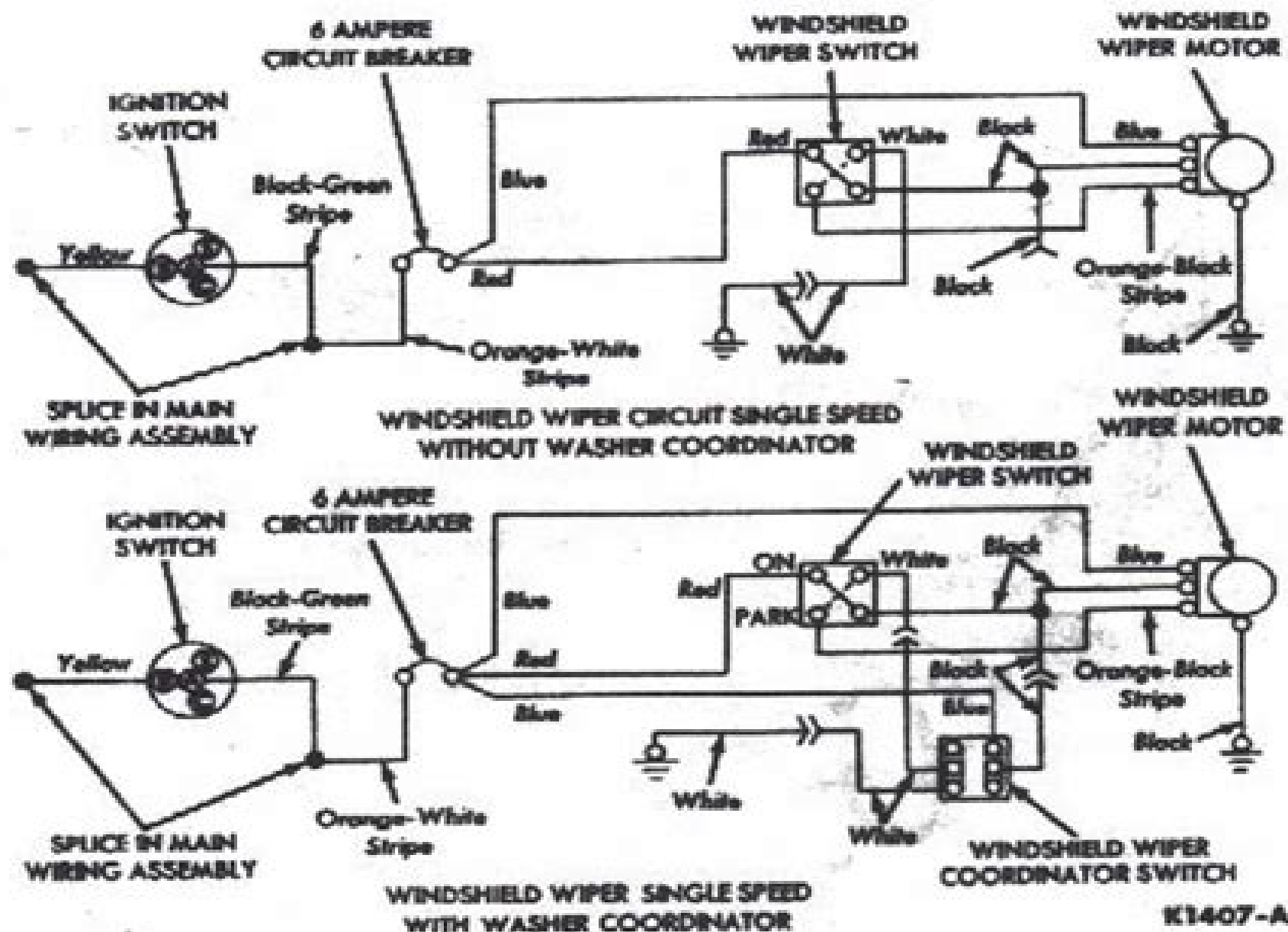
FIG. 89—Single-Speed Wiper Motor Installation Wiring Diagram
